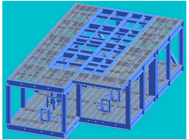
PDMS Model of Chemical Injection Package
